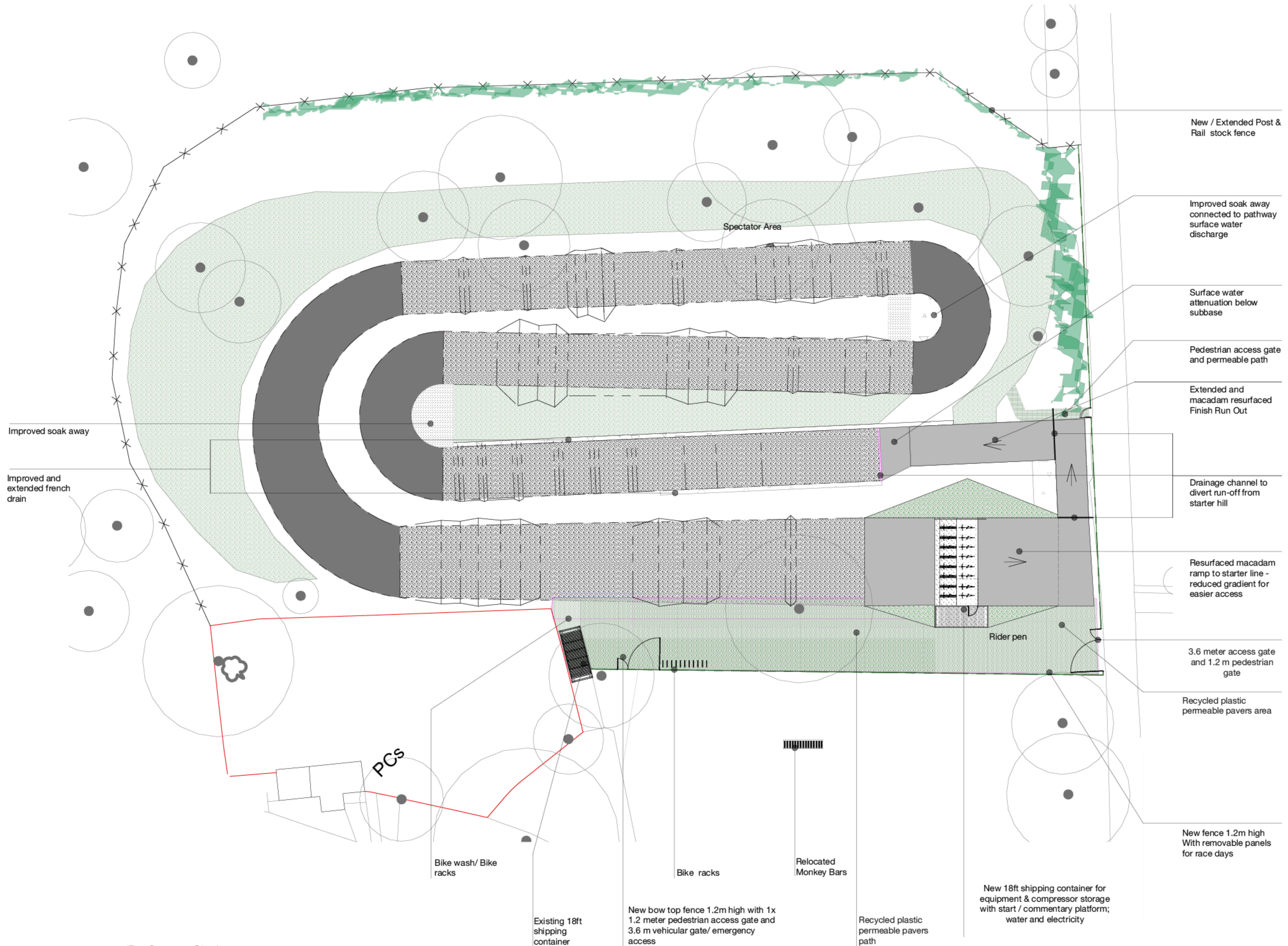
1 Concept Site Layout Scale: 1:200
