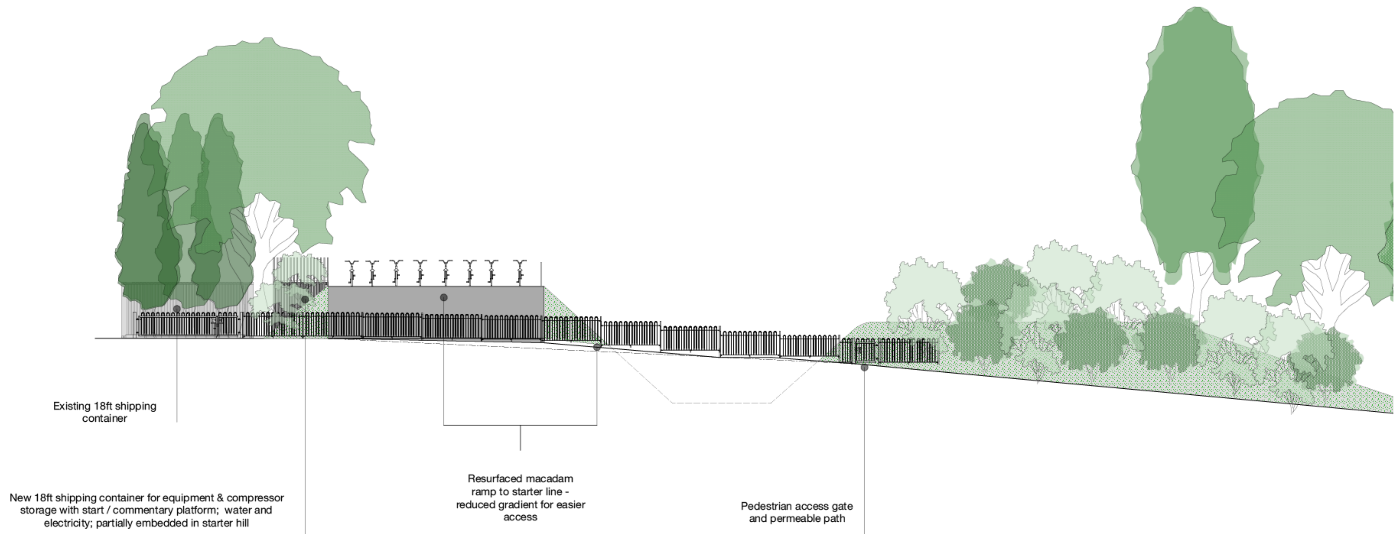
2 Concept Site Elevation A Scale: 1:100
